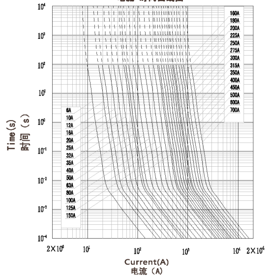
Time-Current Characteristics 电流-时间曲线图
