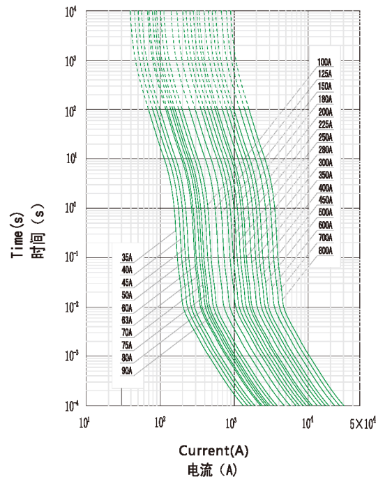
Time-Current Characteristics 电流-时间曲线图
